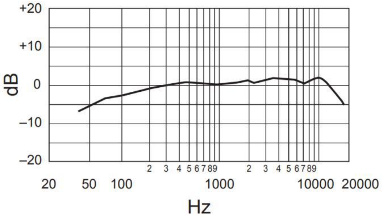
Frequency Response
