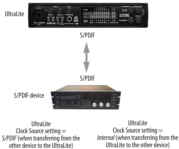
Figure 3-6: The setup for synchronizing a S/PDIF device with the UltraLite. Sync is achieved via the digital I/O connection itself. In this case, you have to choose S/PDIF as the UltraLite's clock source when recording from the other device.
