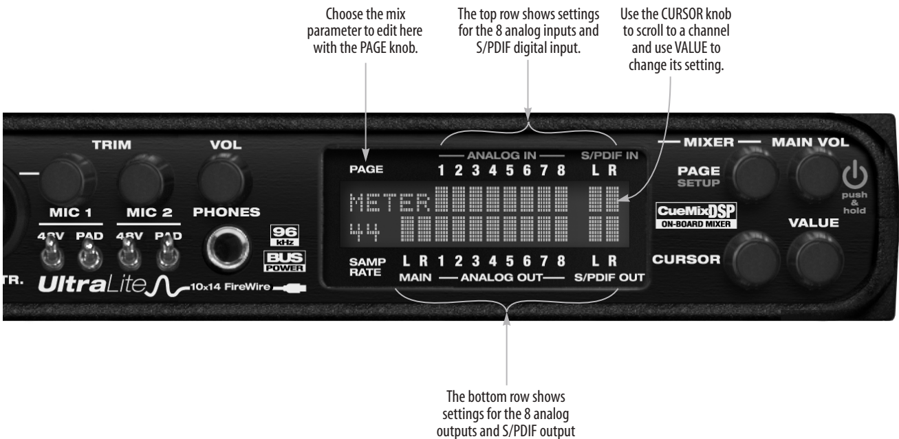
Figure 6-1: The UltraLite front panel controls.
