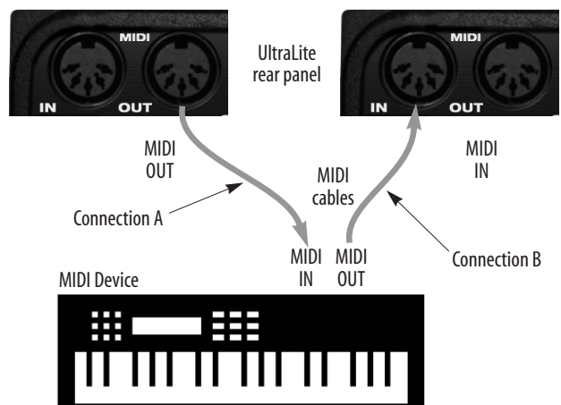
Figure 3-2: Connecting a MIDI device to the UltraLite.
