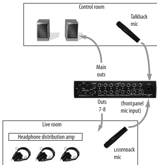
Figure 11-2: Typical hardware setup for Talkback and Listenback.
