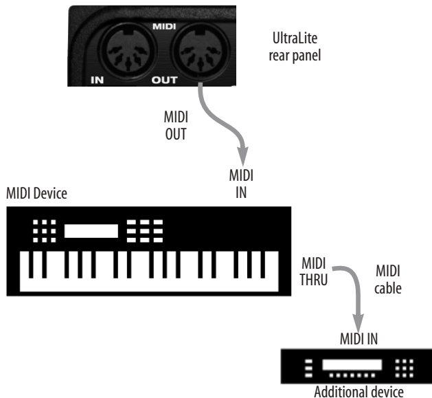
Figure 3-3: Connecting additional devices with MIDI THRU ports.
