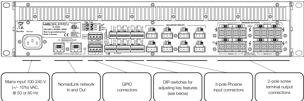
Figure 4.2: C Series rear panel layout
