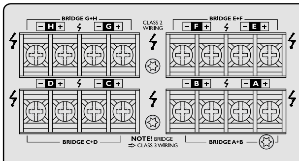
Figure 5.4.2: Screw terminal speaker output field
