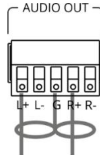
Figure 5: Connecting to an Unbalanced Stereo Audio Acceptor
