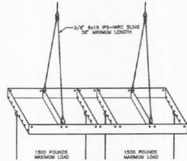
FIGURE 25c — Suggested Rigging Configurations for the Two-Column MT-4A/MT-2A Grid
