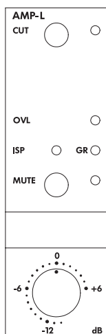
Controls on AMP-L module
