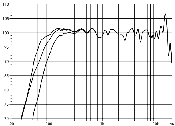
MAX frequency response (linear setup, free field) CPL +5, standard and CUT
