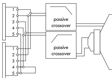
Connector wiring (4-wire operation with EP5 connectors)
