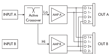
P1200A with ampMAX, "2-Way Active" mode
