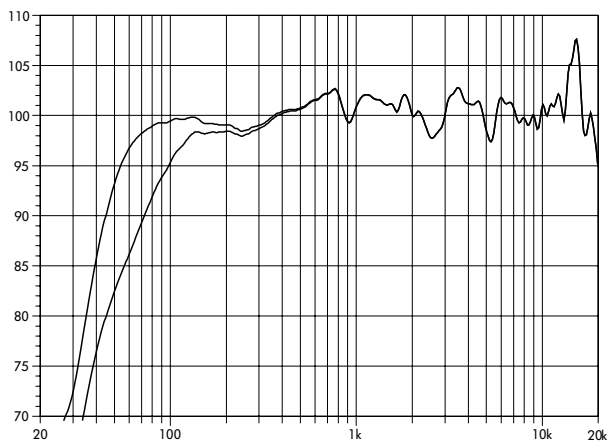
MAX frequency response (MAX setup, floor coupling), standard and CUT
