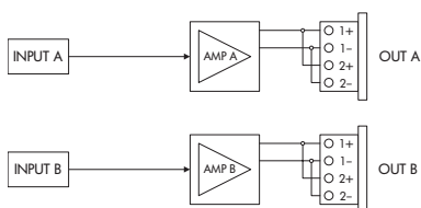
P1200A with ampMAX, "Passive" mode
