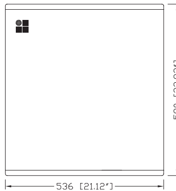
MAX cabinet dimensions in mm [inch]
