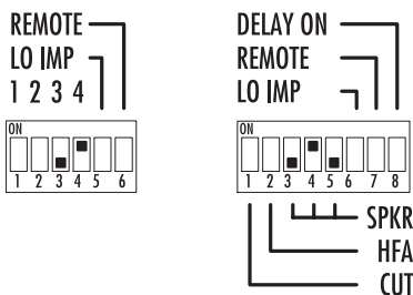
E-PAC version 1, E-PAC version 2 E-PAC configuration for "Linear" mode
