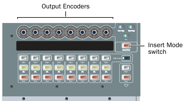
Encoders and Insert mode switch in the Output section
