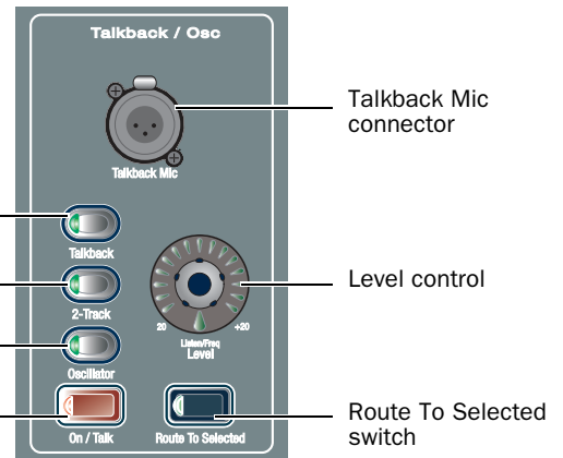
Talkback controls in the Talkback/Osc section
