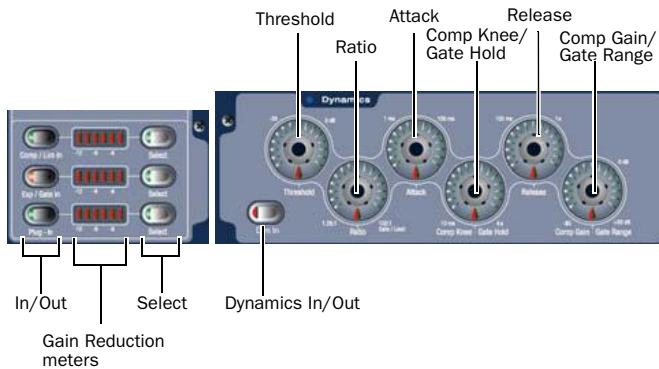
ACS Dynamics section and controls
