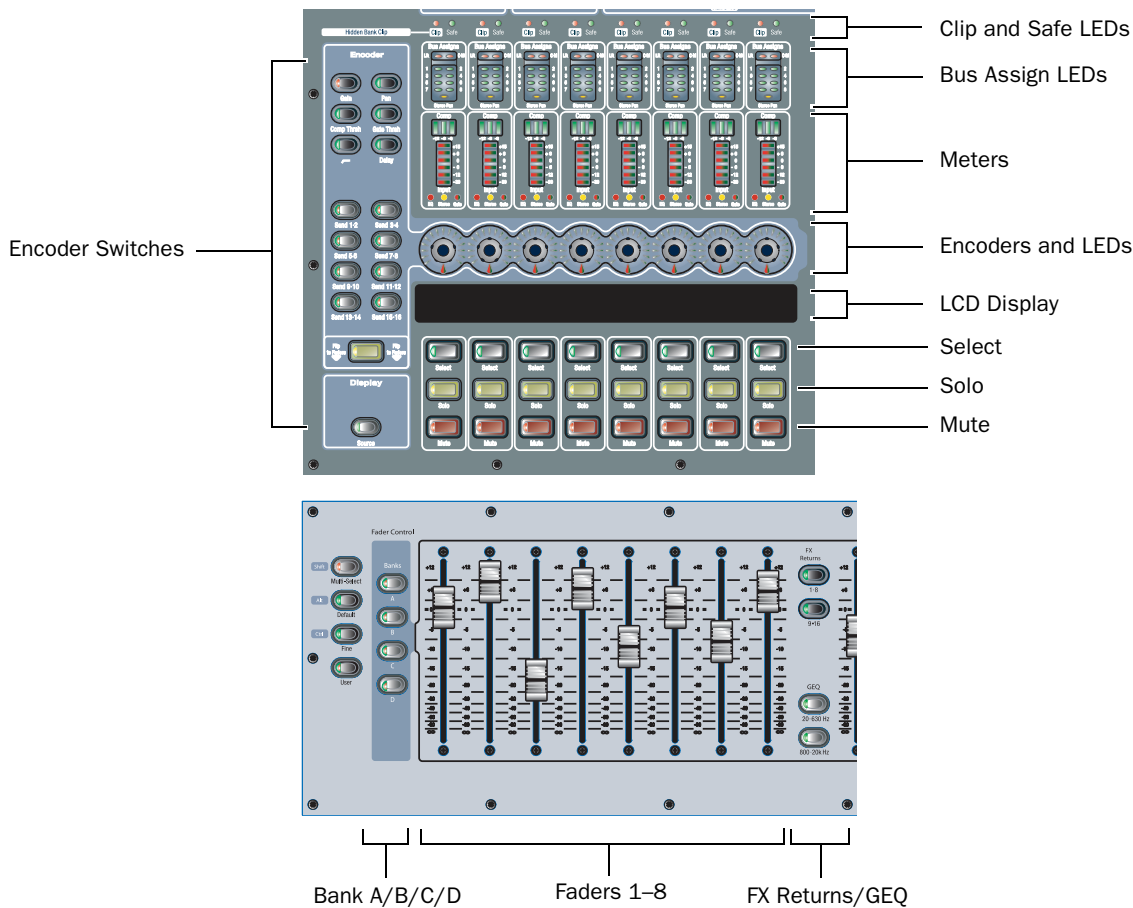
Figure 12. Input controls (Input Channels 1–8 shown)
