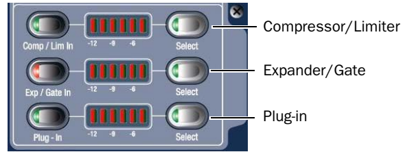
Selected Channel Gain Reduction meters
