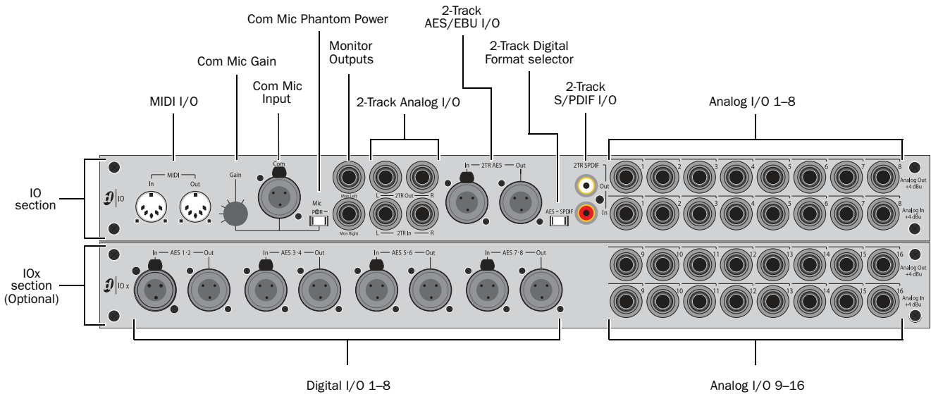
Figure 10. Audio connectors on FOH Rack, showing standard IO connectors (top) and optional IOx connectors (bottom)
