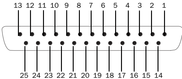
Pinout for Profile DB25F GPI Output port (looking at back of console)
