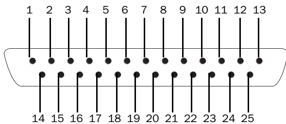
Pinout for Profile DB25M GPI Input port (looking at back of console)
