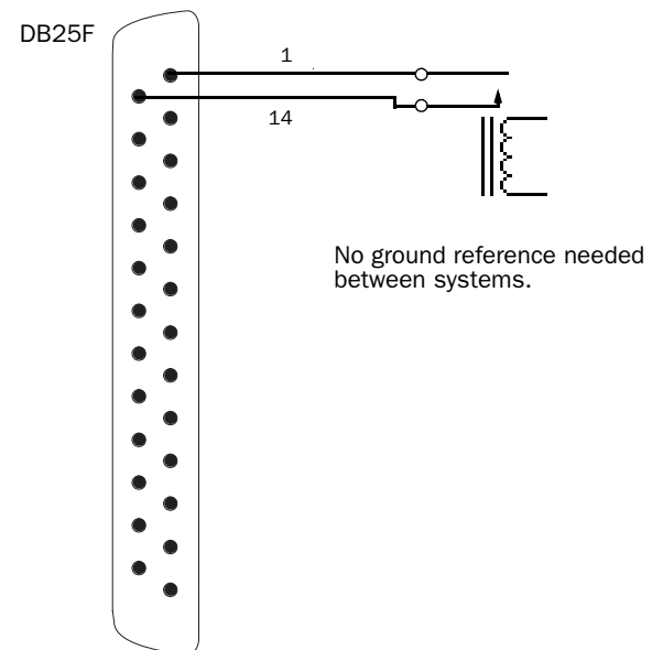
Pinout for Profile DB25F GPI Output port (looking at back of console)
