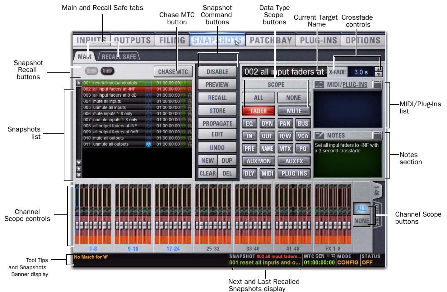
Figure 17. Sections of the Snapshots page
