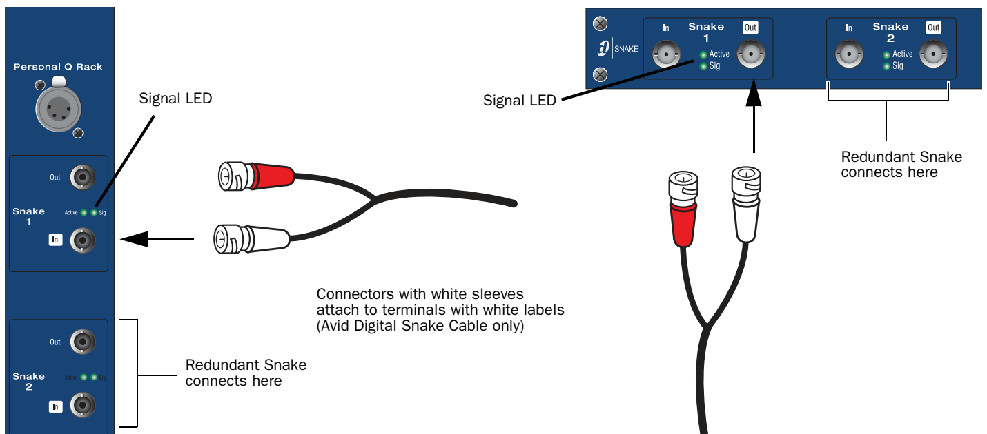
Figure 7. Detail of Digital Snake cable connection between Stage Rack (left) and FOH Rack (right)
