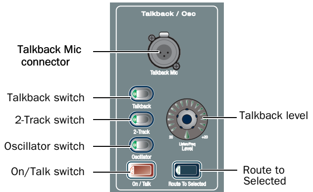
Talkback microphone connector and controls
