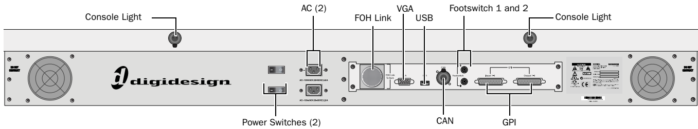
Figure 21. D-Show Profile back panel
