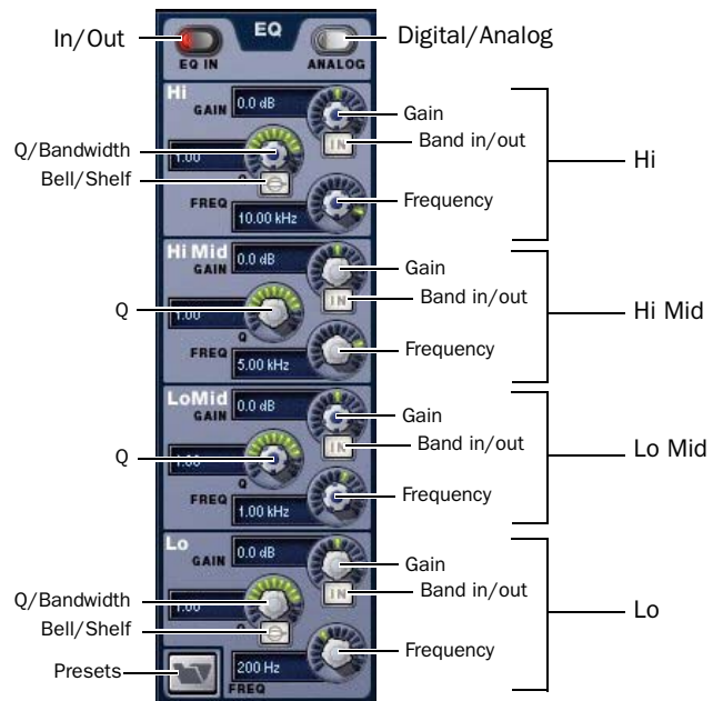
EQ controls in the software screen (4-band Input Channel EQ shown)
