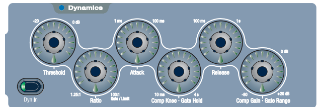
Dynamics section and controls
