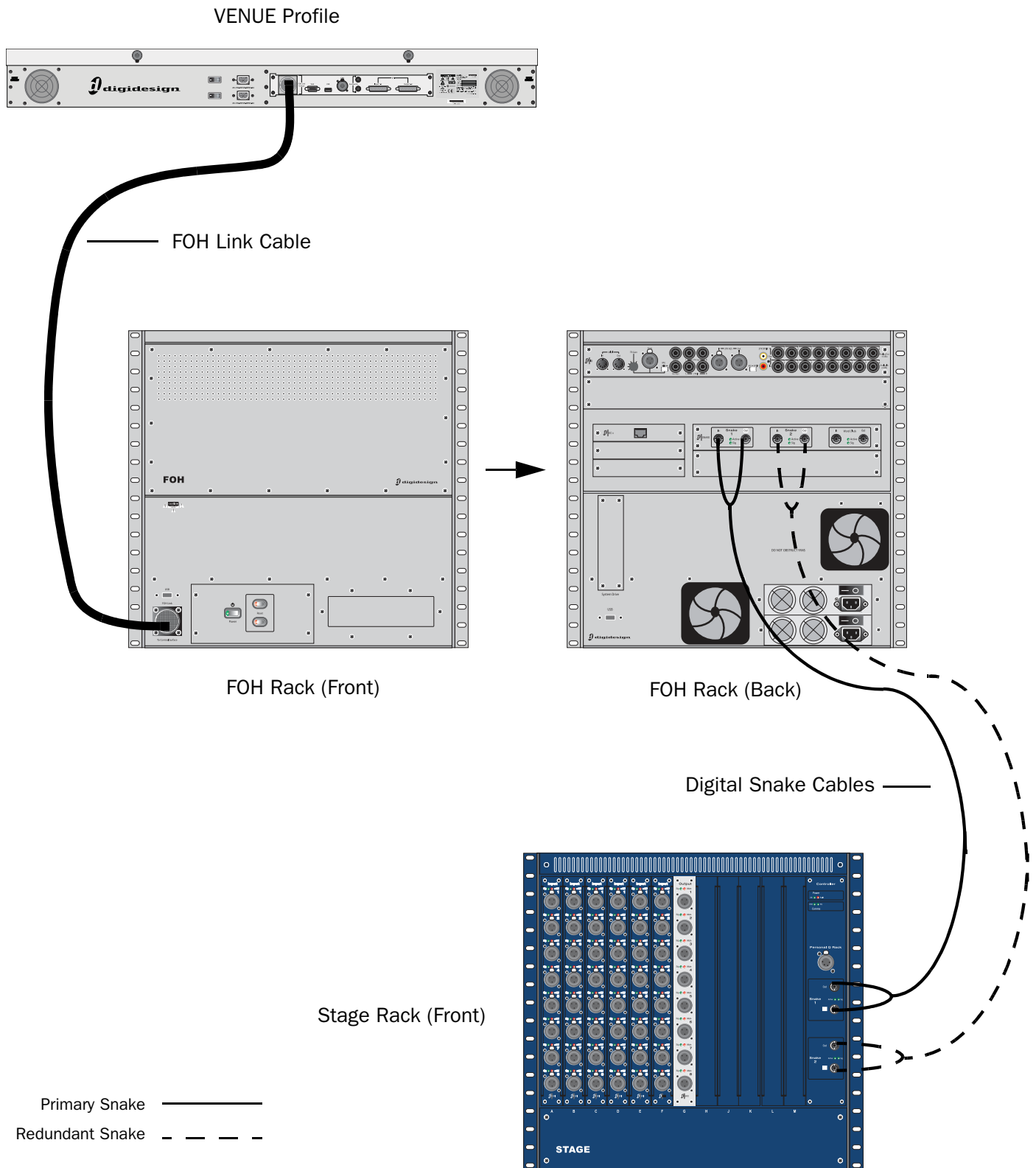
Figure 5. VENUE Profile system component connections
