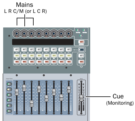
Bus control while Cue on Mains is enabled
