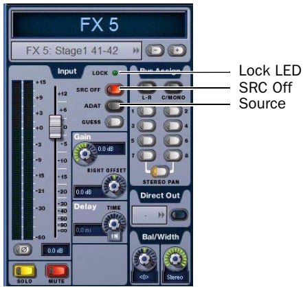
Input controls for a DSI channel
