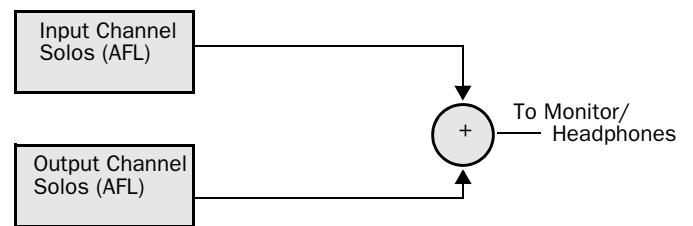
No Level Trim in AFL mode
