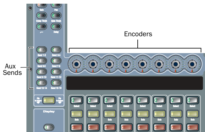
Encoder assignment switches for input channels
