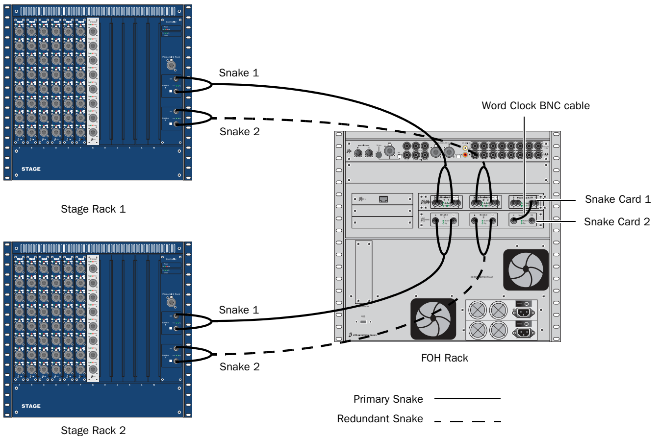
Figure 8. Digital Snake cable and word clock connections for fully redundant system with 2 Stage Racks
