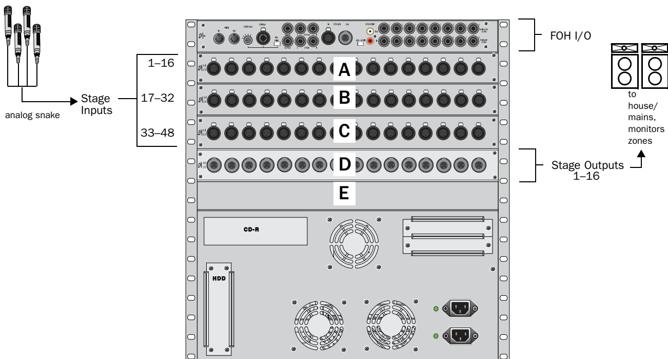
Figure 3. Mix Rack audio connectors and I/O slots (A-E) for stage inputs and outputs
