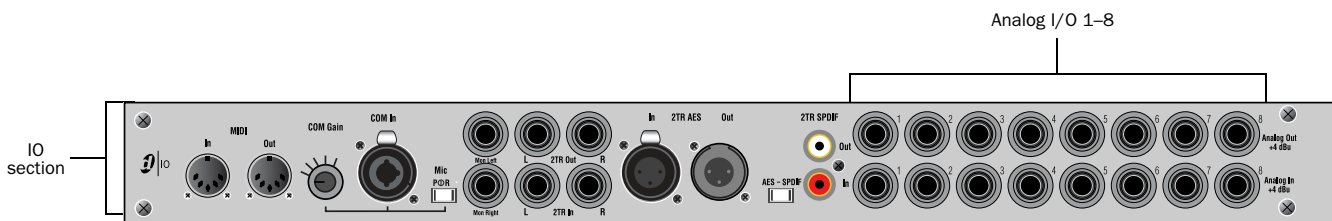
Figure 16. Hardware insert patch points on Mix Rack and FOH Rack, showing standard mix position (FOH) I/O connectors
