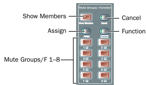
Mute Groups section
