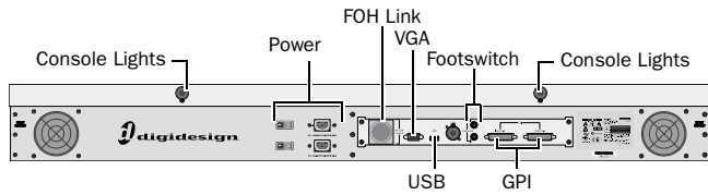
VENUE Profile back panel and connectors
