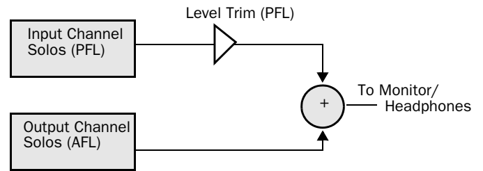
Level Trim in PFL mode
